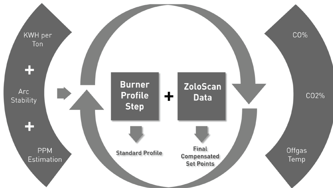
Figure 6. Dynamic compensation of carbon and oxygen references by Off Gas measurement.
