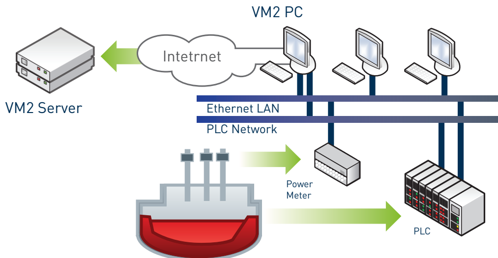
Figure 3. TransformerCare VM2 Remote Monitoring System.
