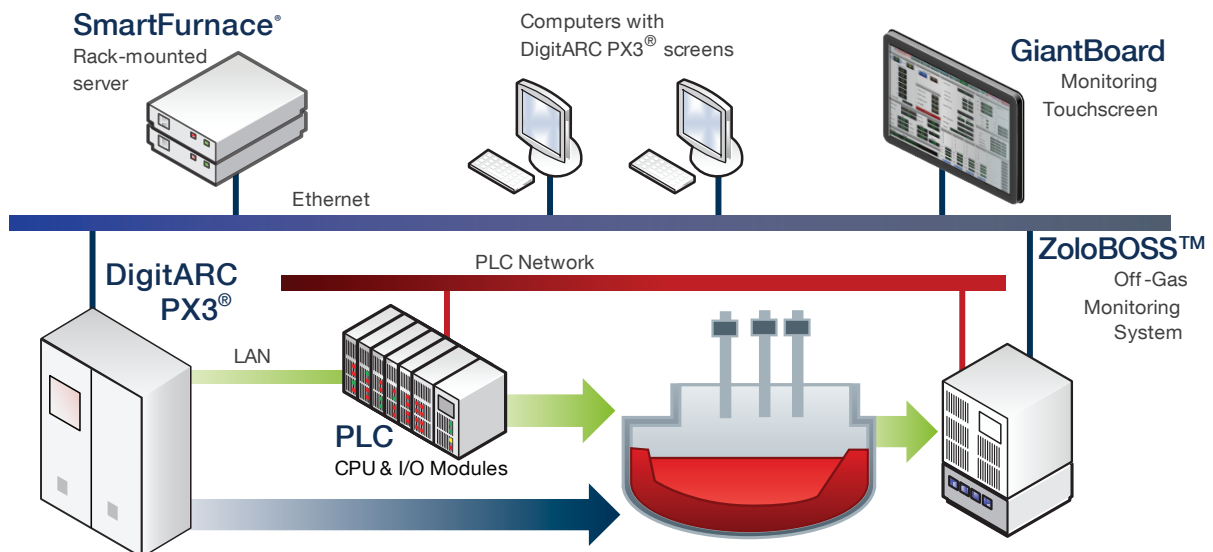
Figure 1. Architecture of the control system
