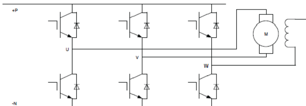
Figure 6. Connection from inverter to DC motor.
